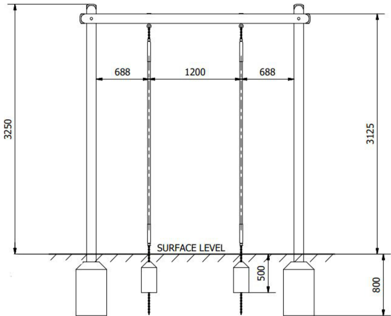
Side Elevation
