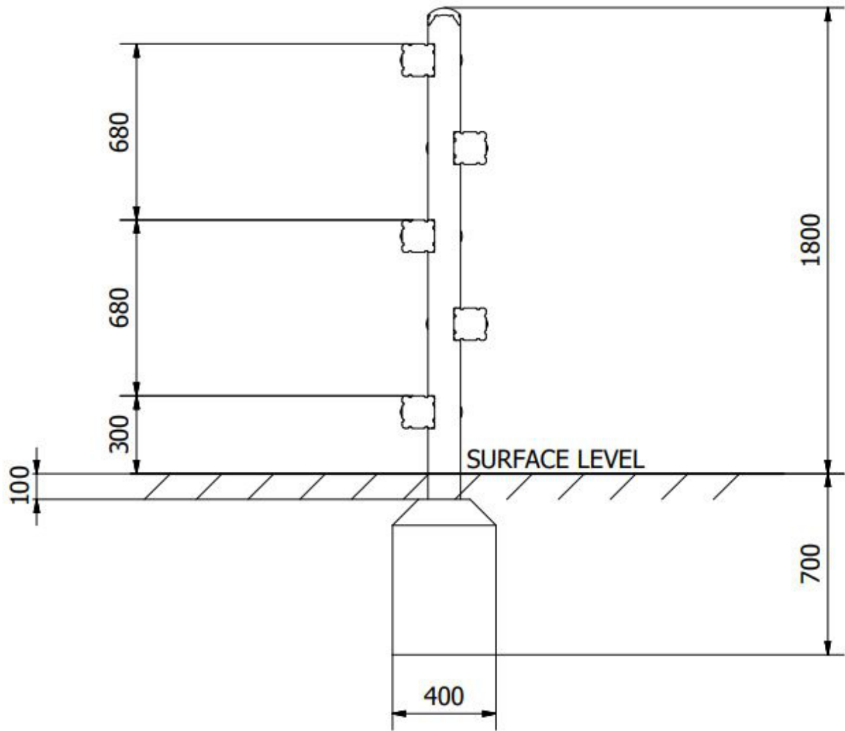
Side Elevation
