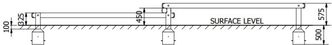
Side Elevation
