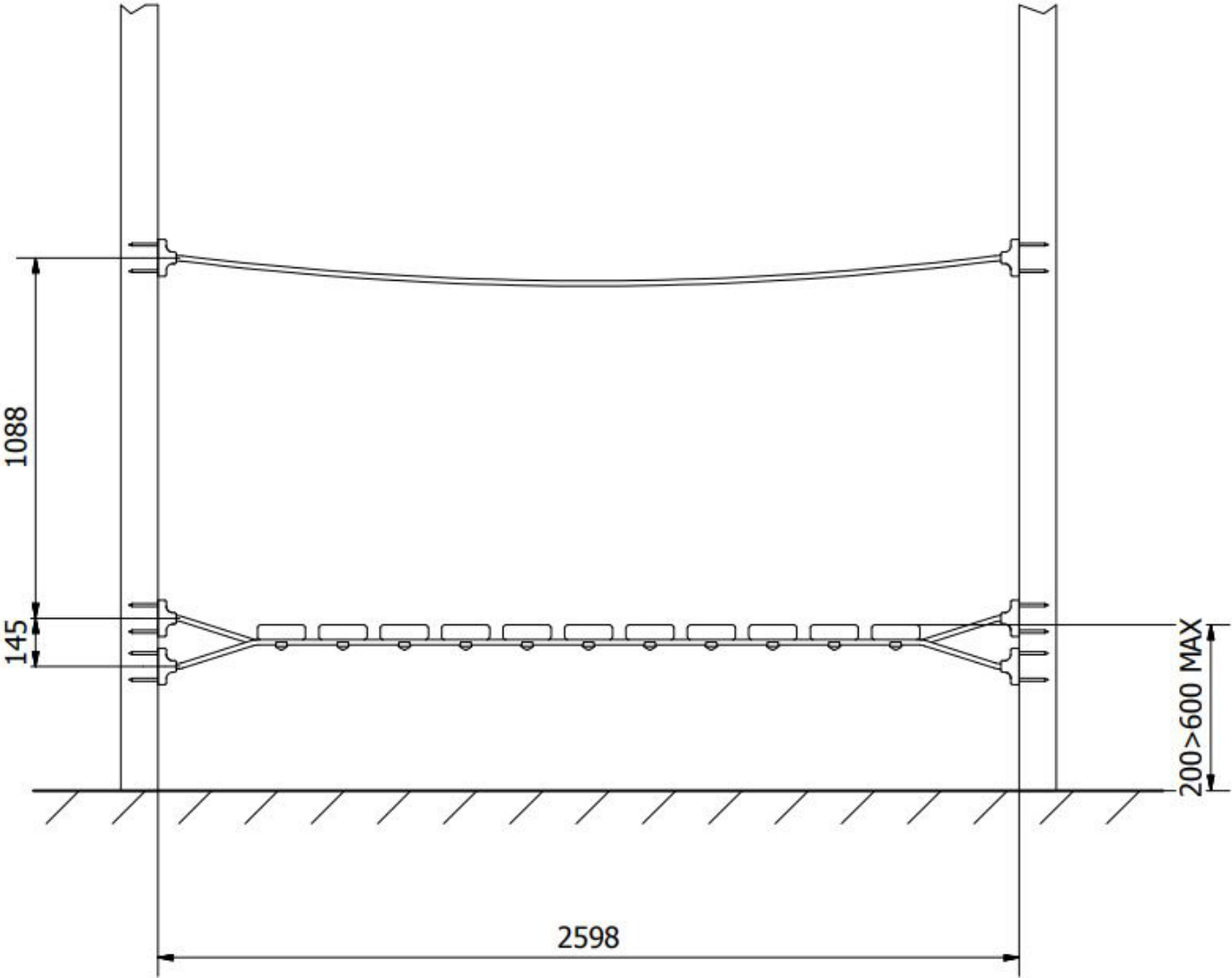
Side Elevation
