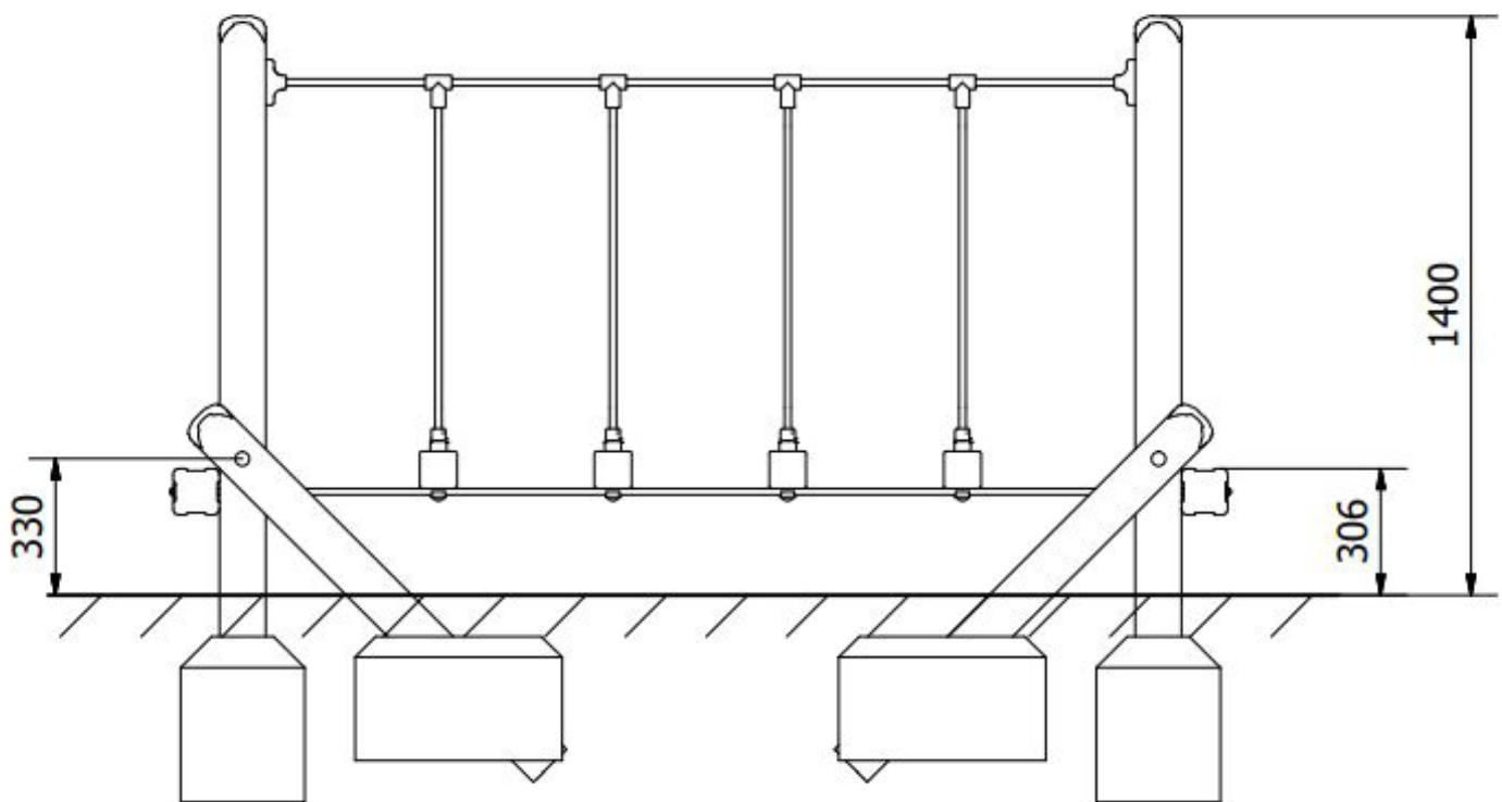
Side Elevation
