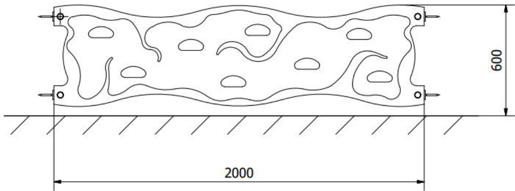
Side Elevation
