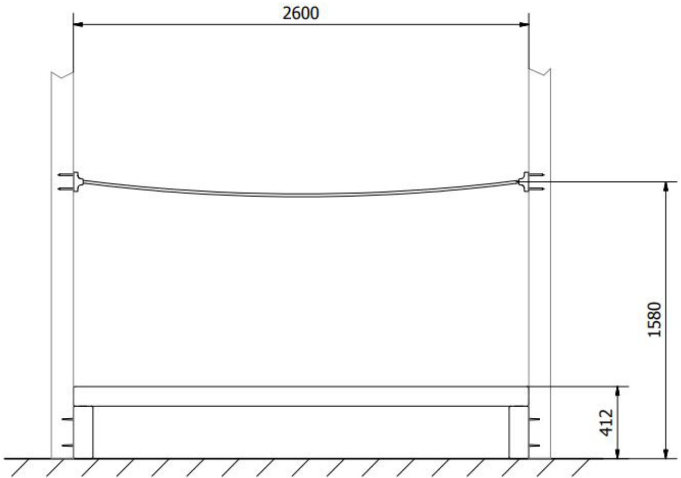
Side Elevation
