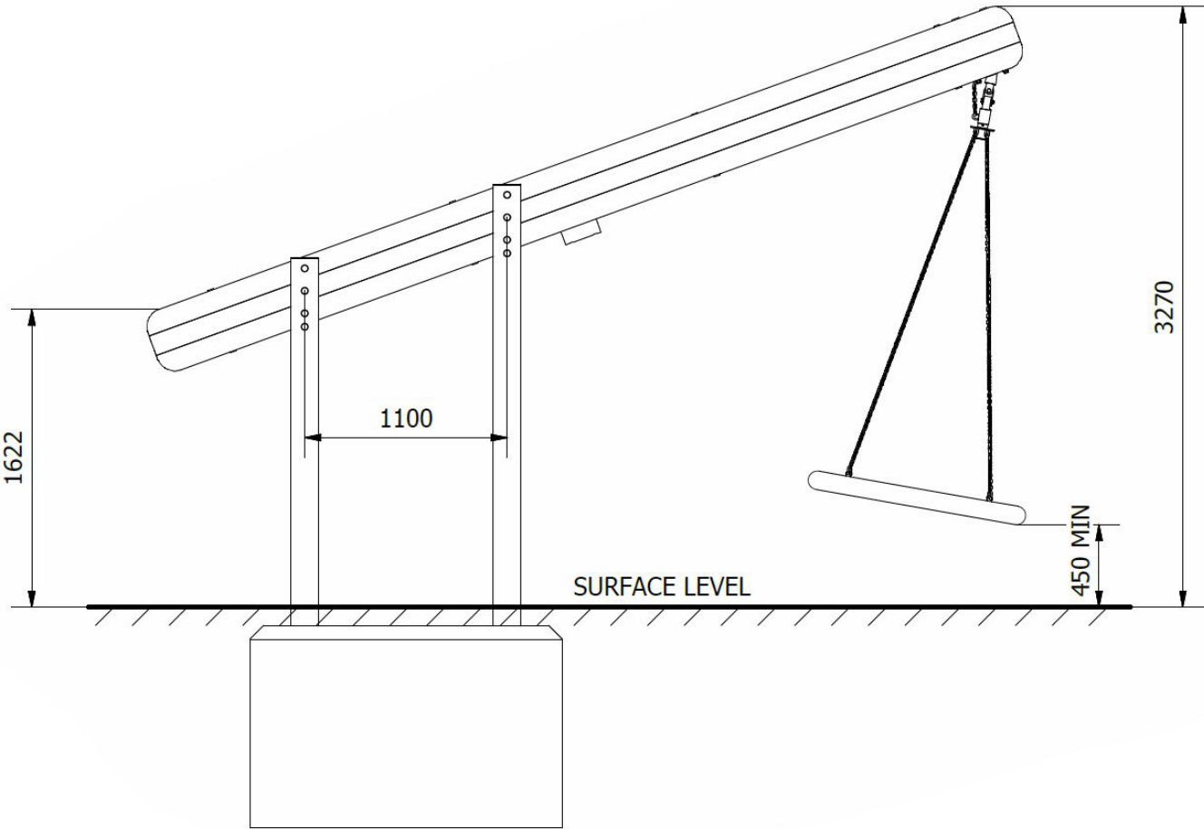
Side Elevation
