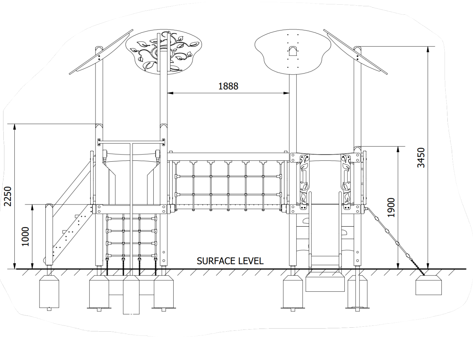
Side Elevation
