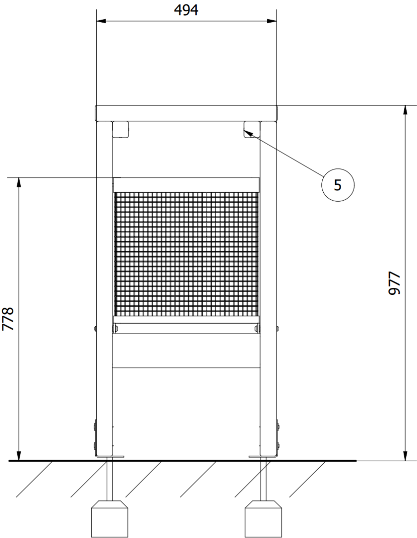
Side Elevation
