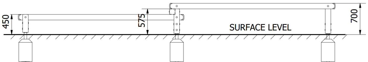
Side Elevation
