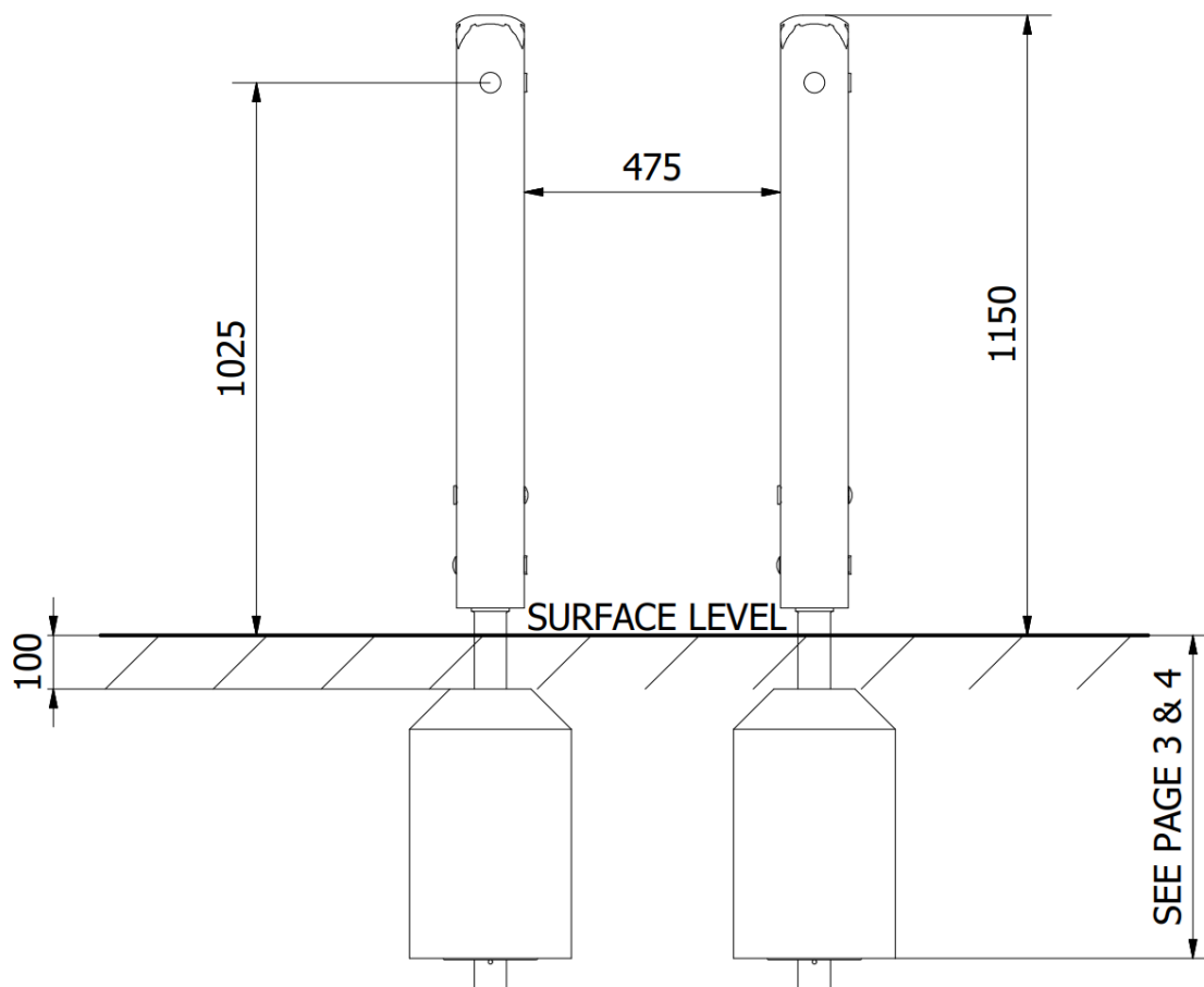
Side Elevation
