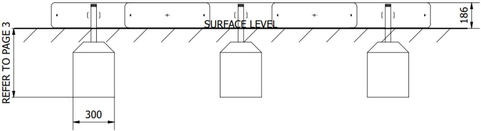
Side Elevation
