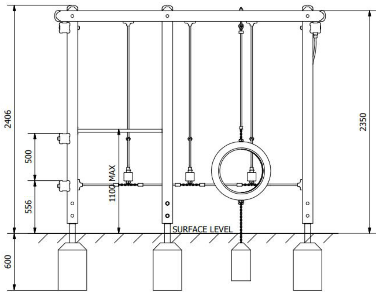
Side Elevation
