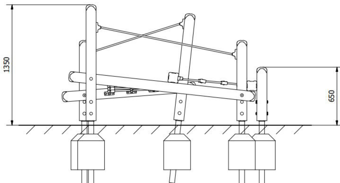
Side Elevation
