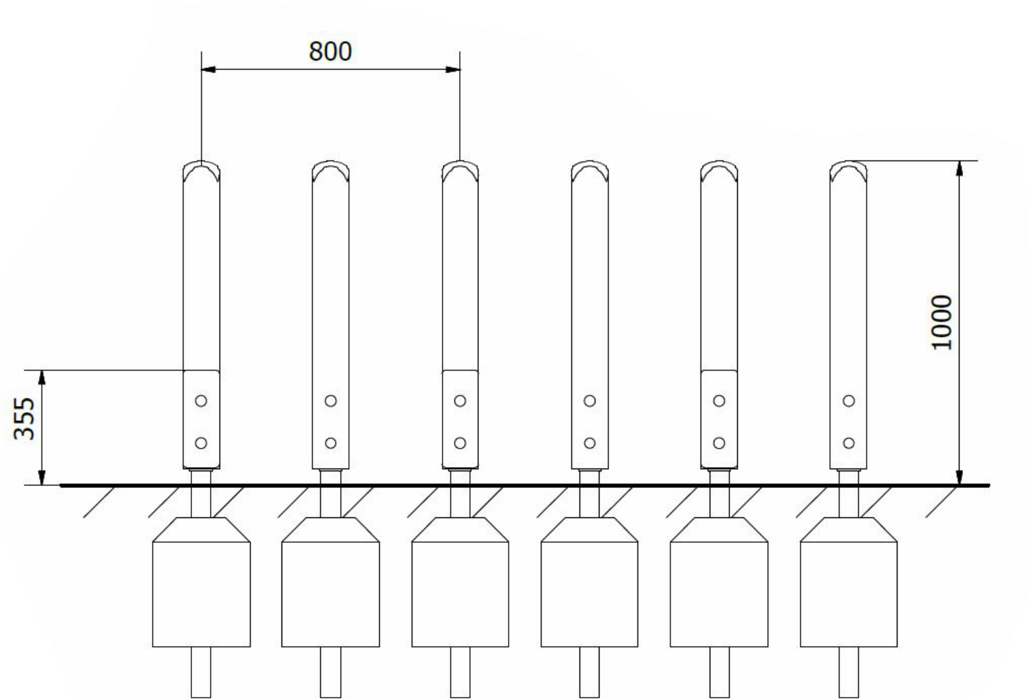
Side Elevation
