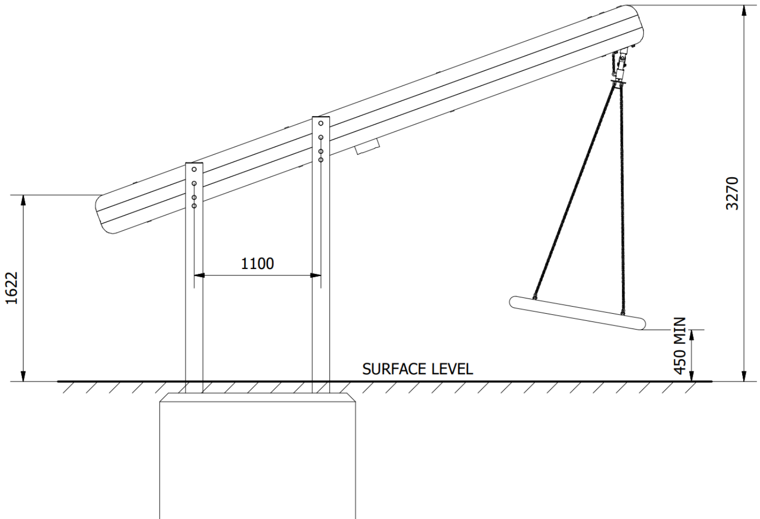
Side Elevation
