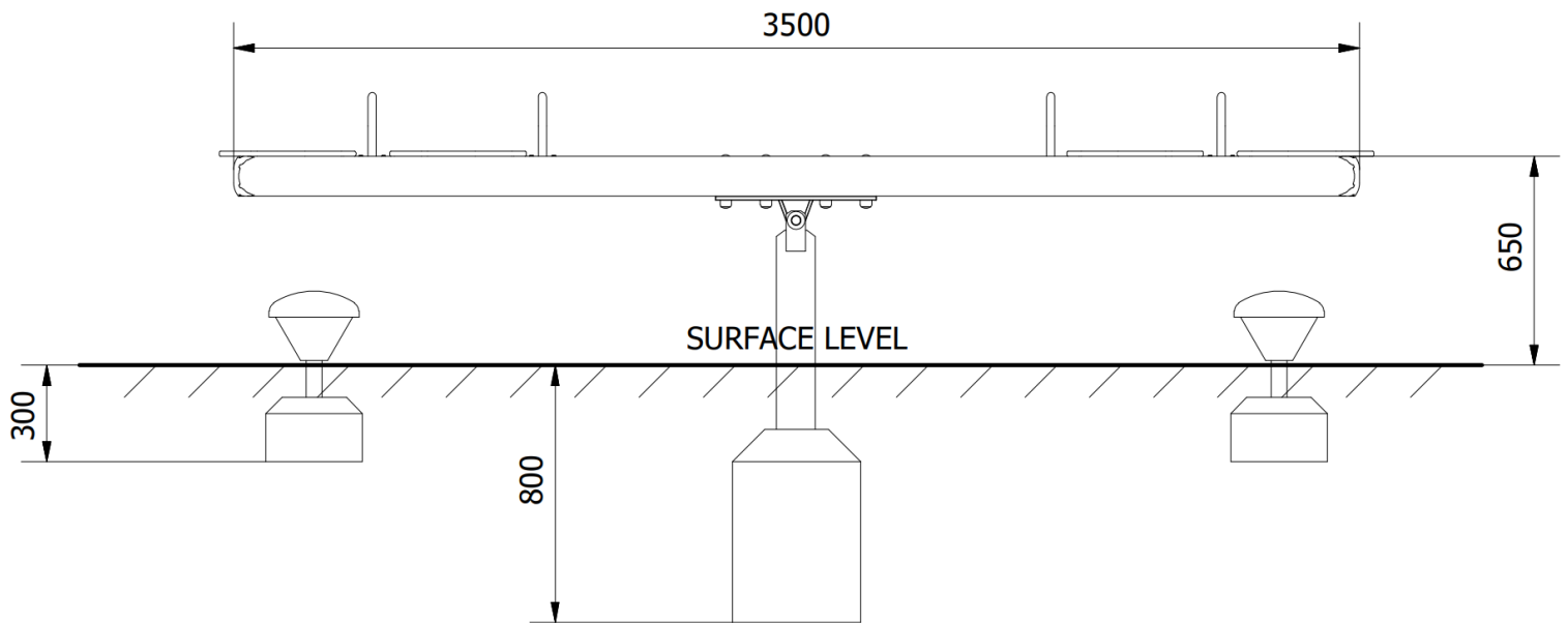
Side Elevation
