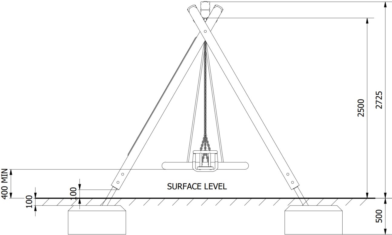
Side Elevation
