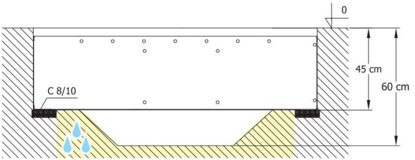
Side Elevation
