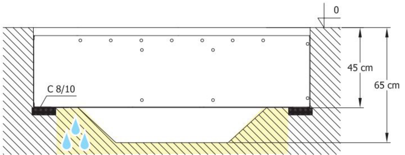
Side Elevation
