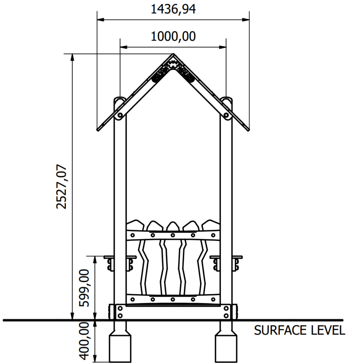
Side Elevation
