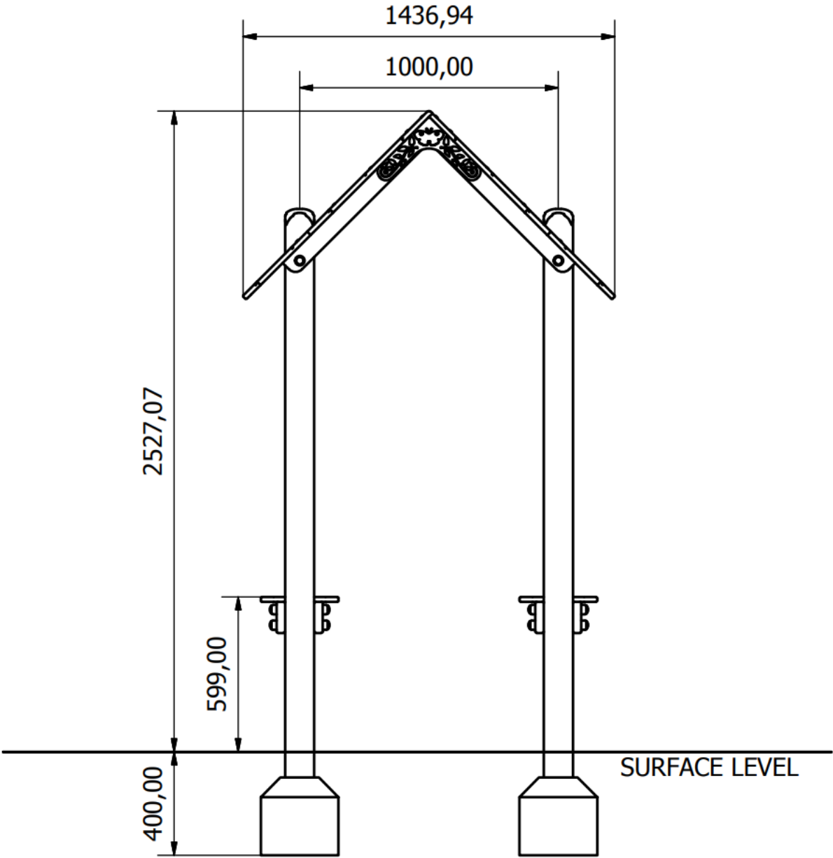
Side Elevation
