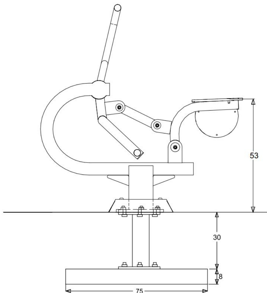
Side Elevation
