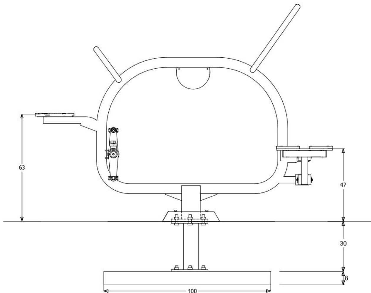
Side Elevation
