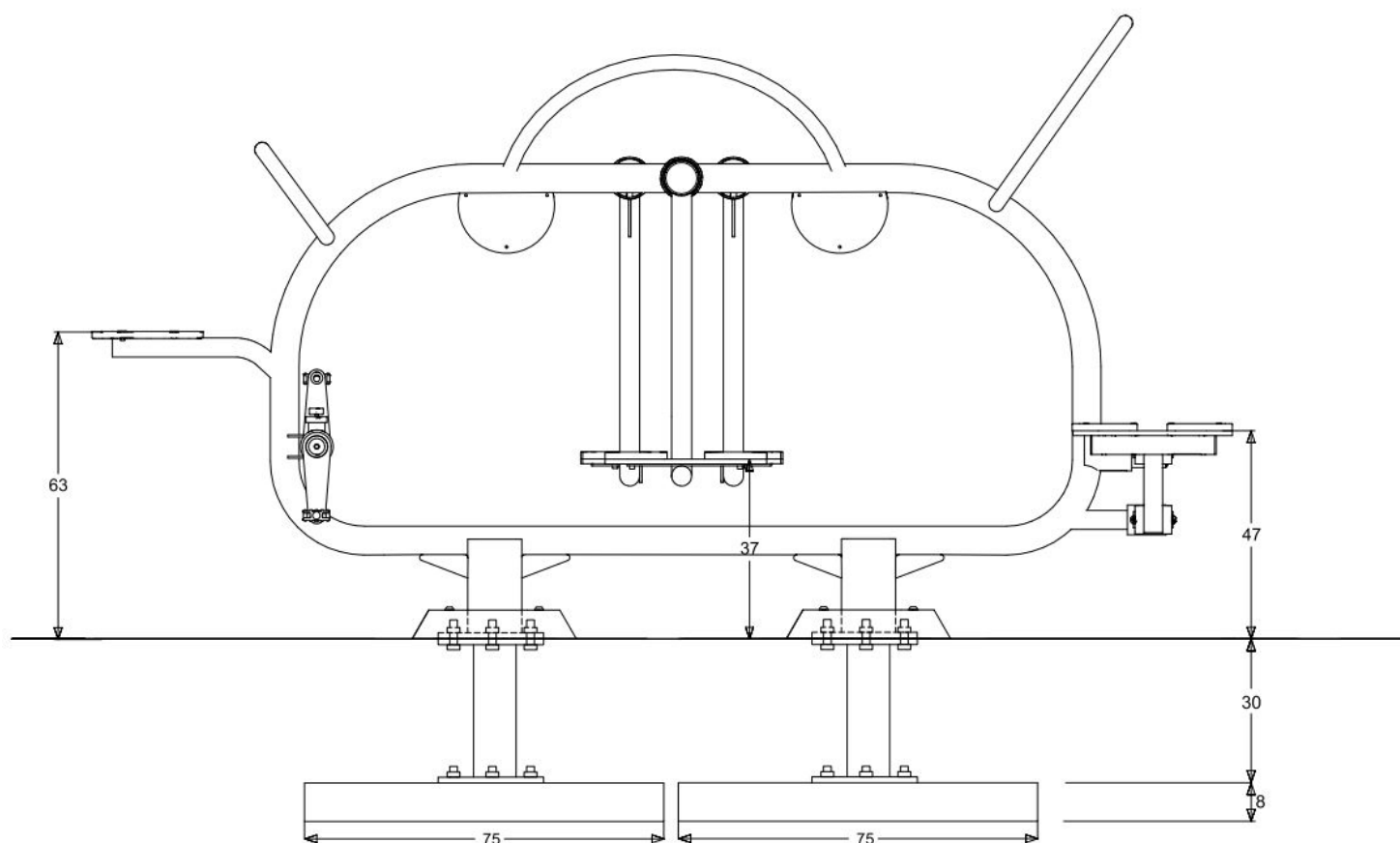
Side Elevation
