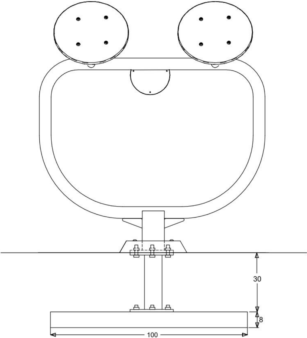
Side Elevation
