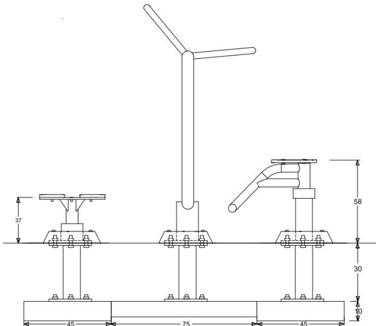
Side Elevation
