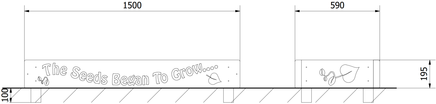
Side Elevation
