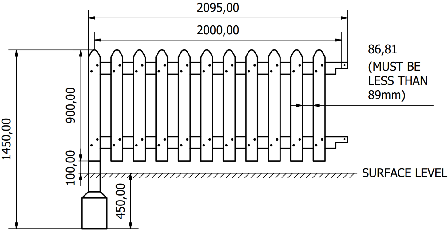
Side Elevation
