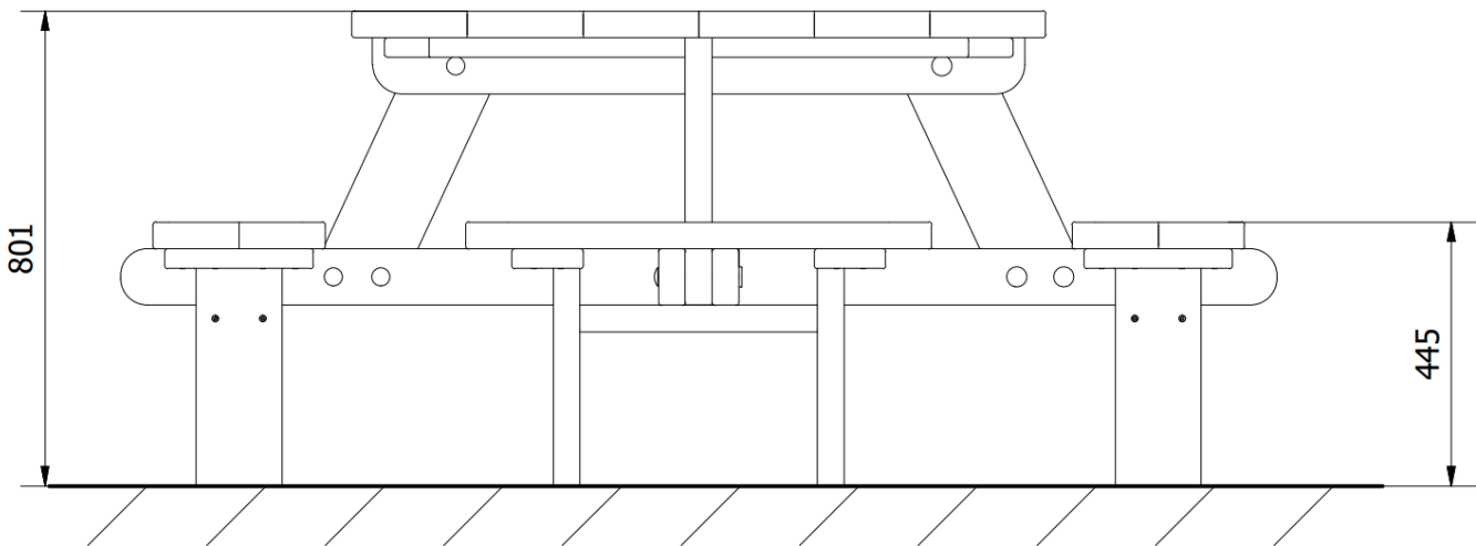
Side Elevation
