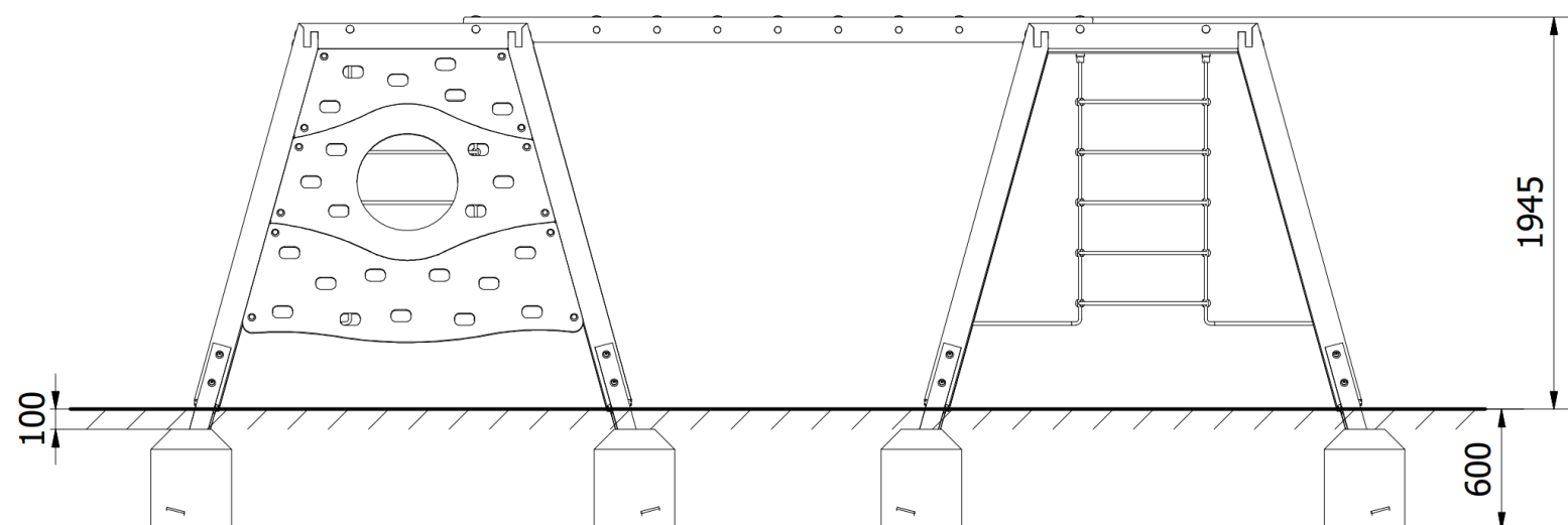
Side Elevation
