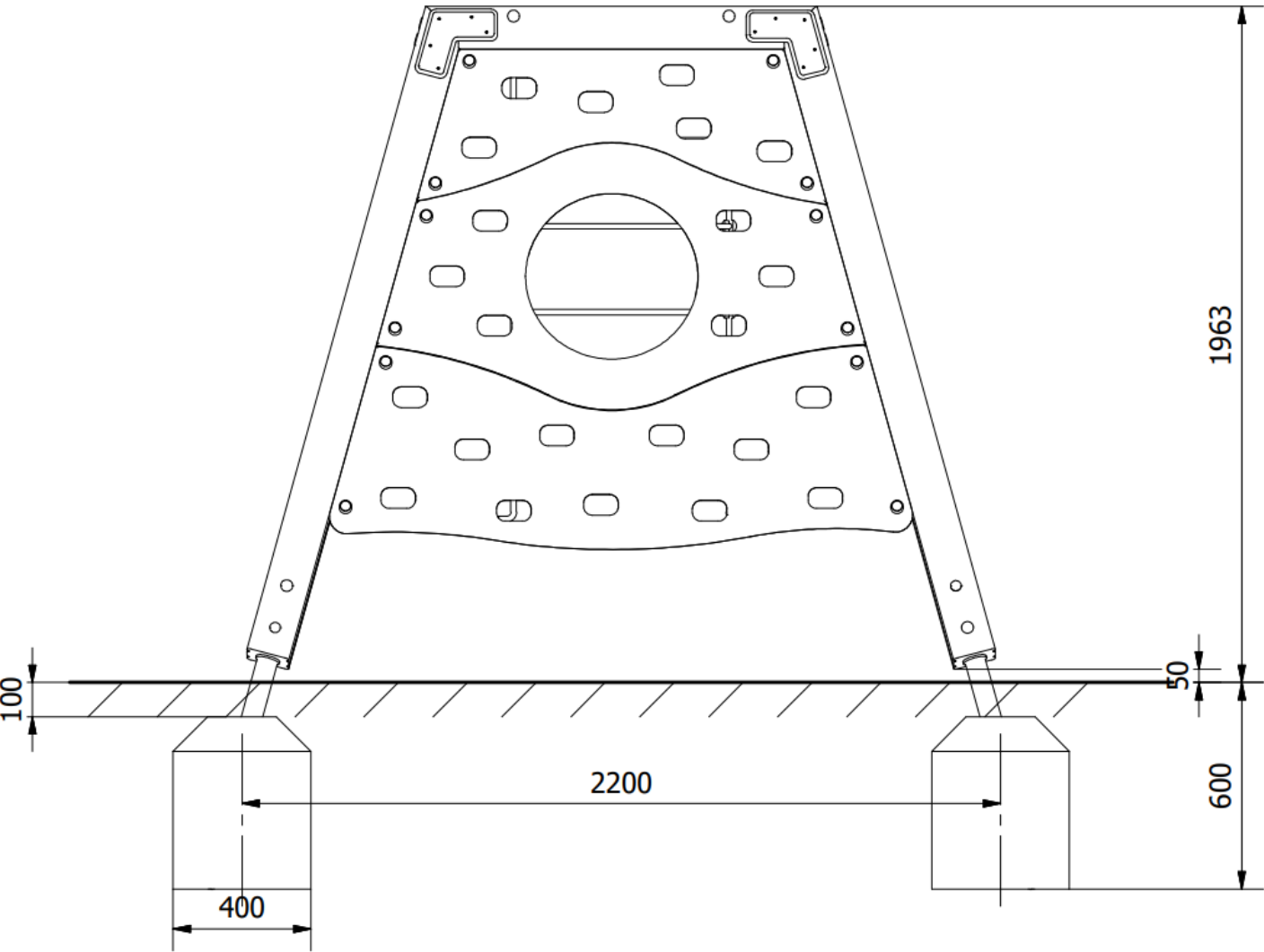
Side Elevation
