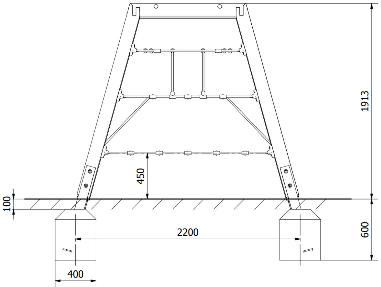
Side Elevation
