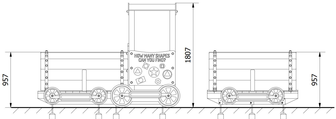
Side Elevation
