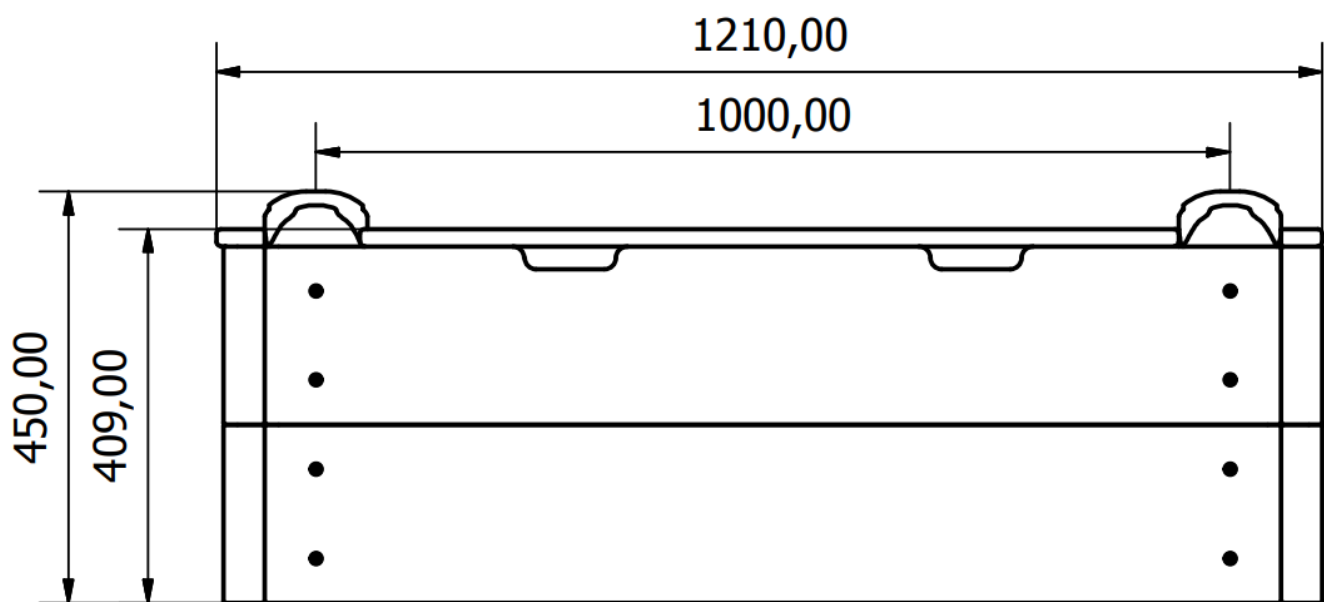
Side Elevation
