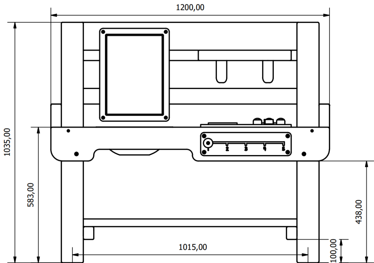
Side Elevation
