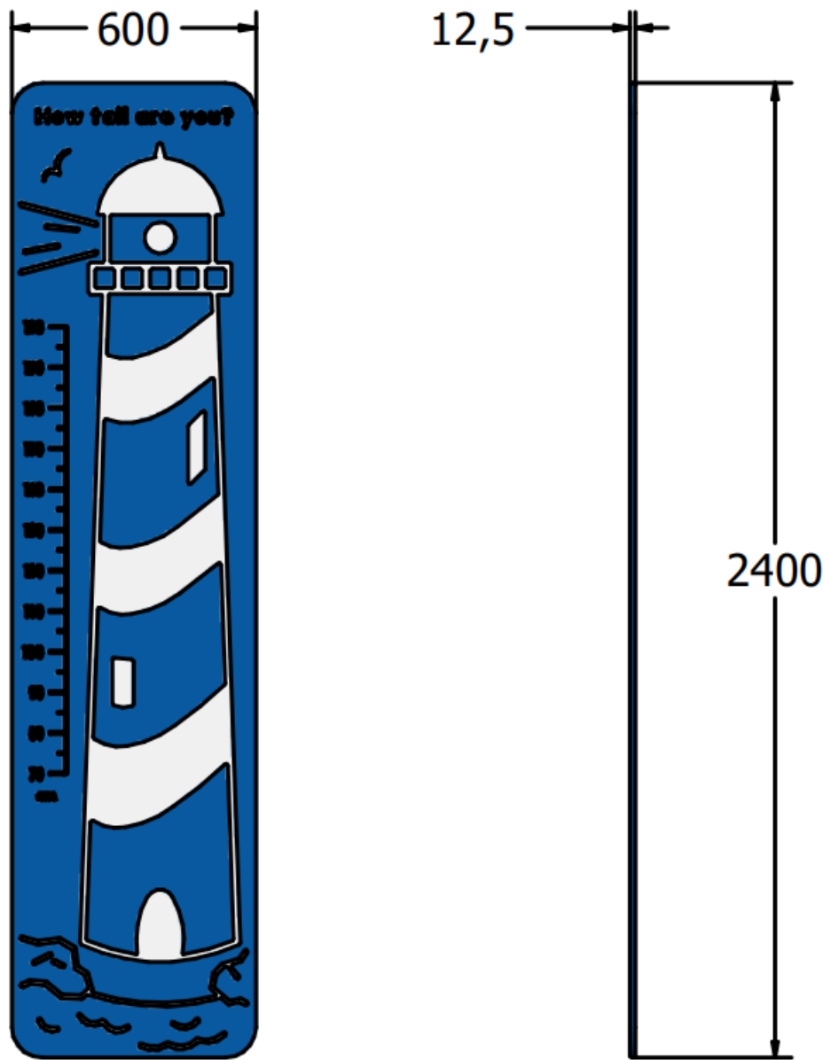
Side Elevation
