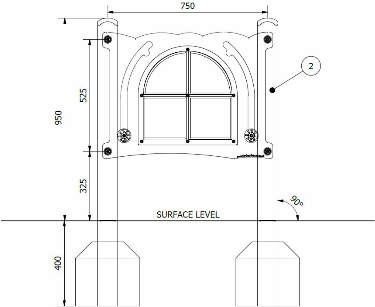
Side Elevation
