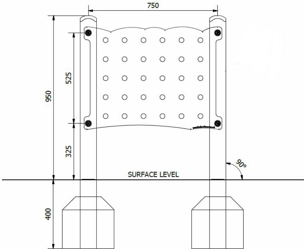
Side Elevation
