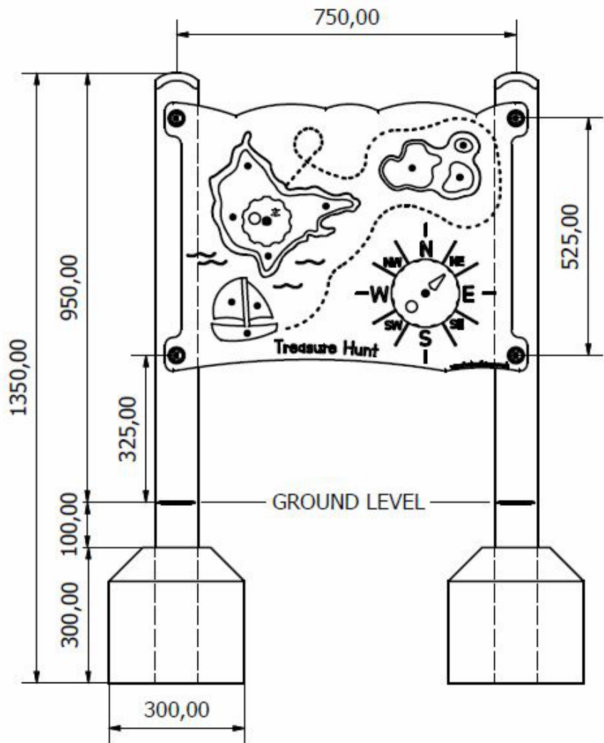
Side Elevation
