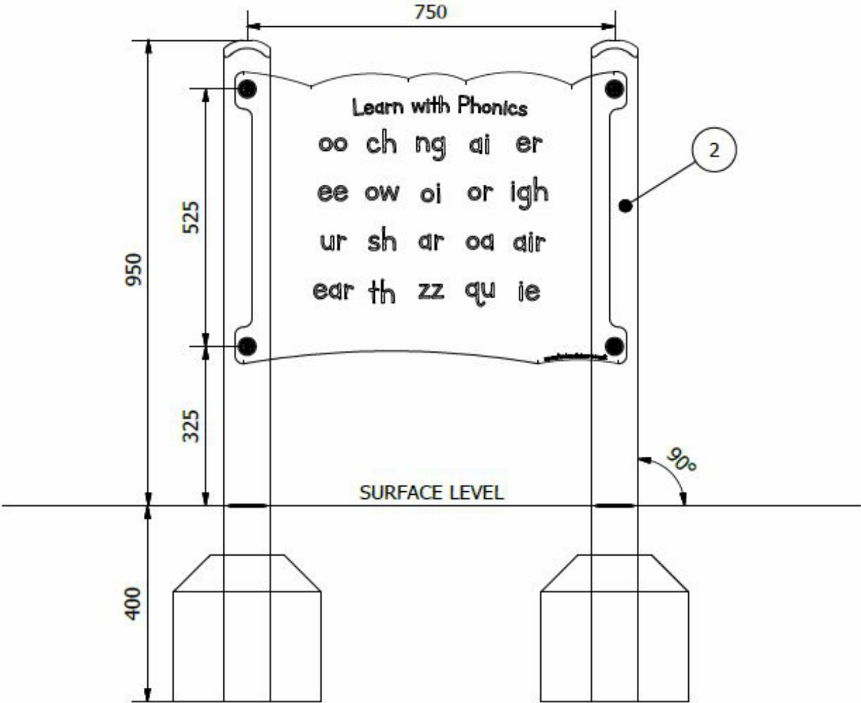
Side Elevation
