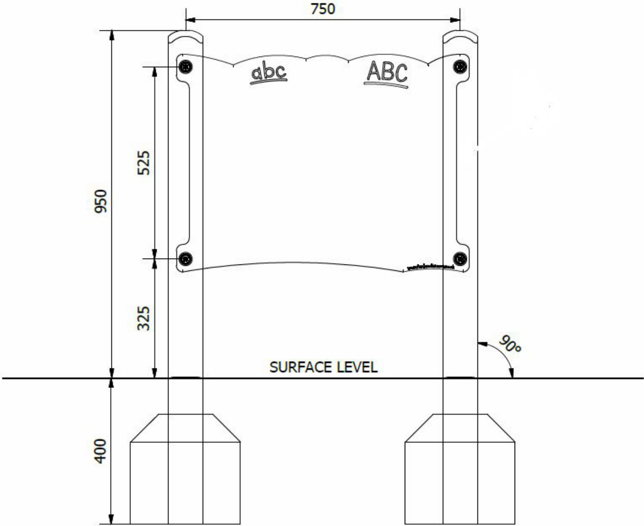
Side Elevation
