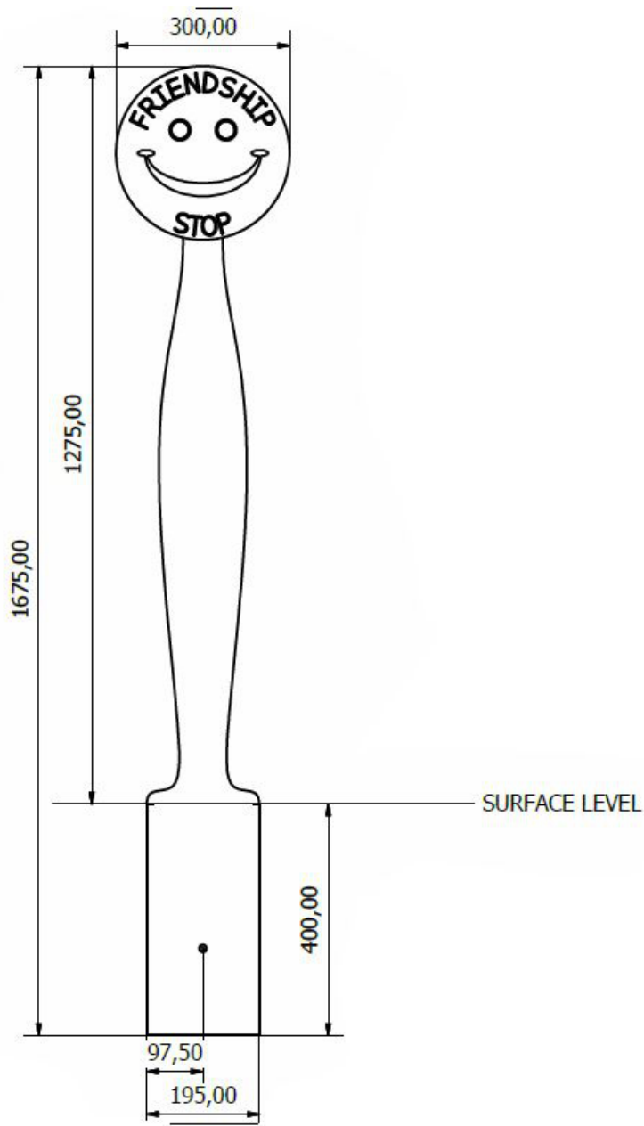
Side Elevation
