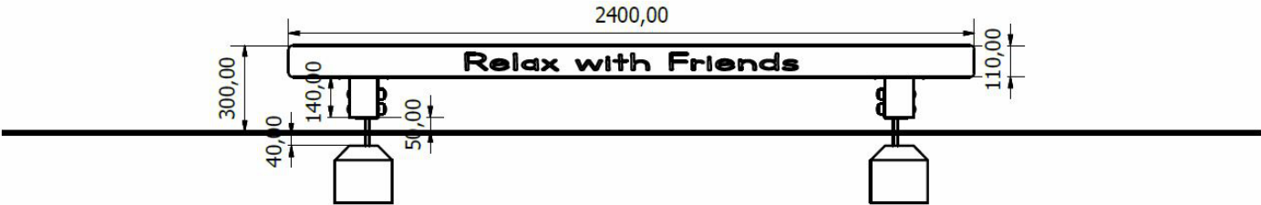
Side Elevation
