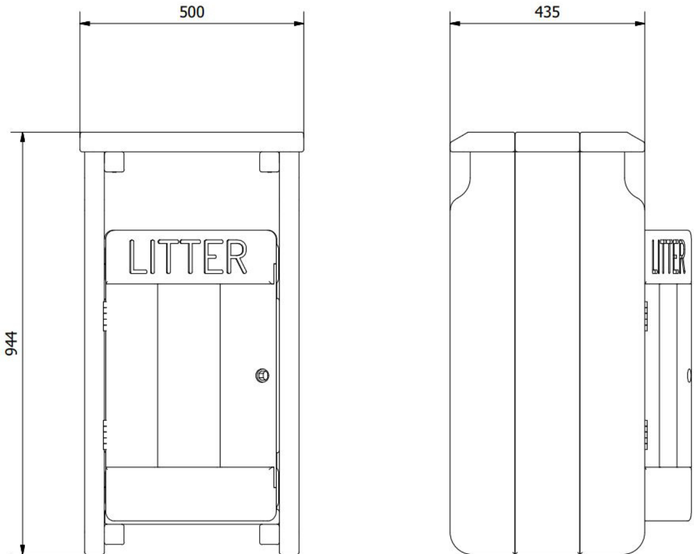
Side Elevation
