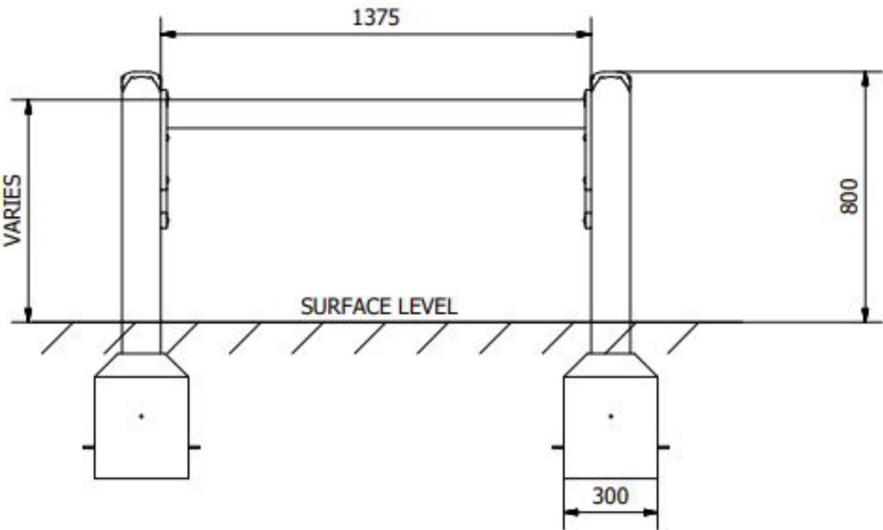
Side Elevation
