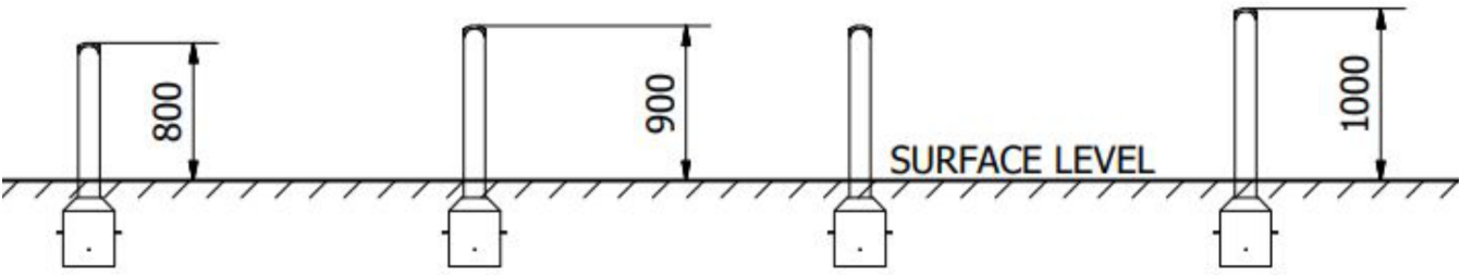
Side Elevation
