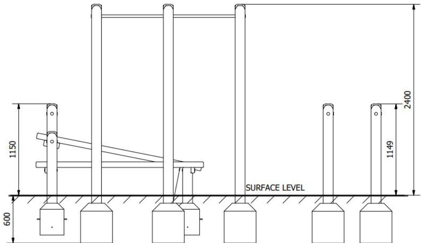
Side Elevation
