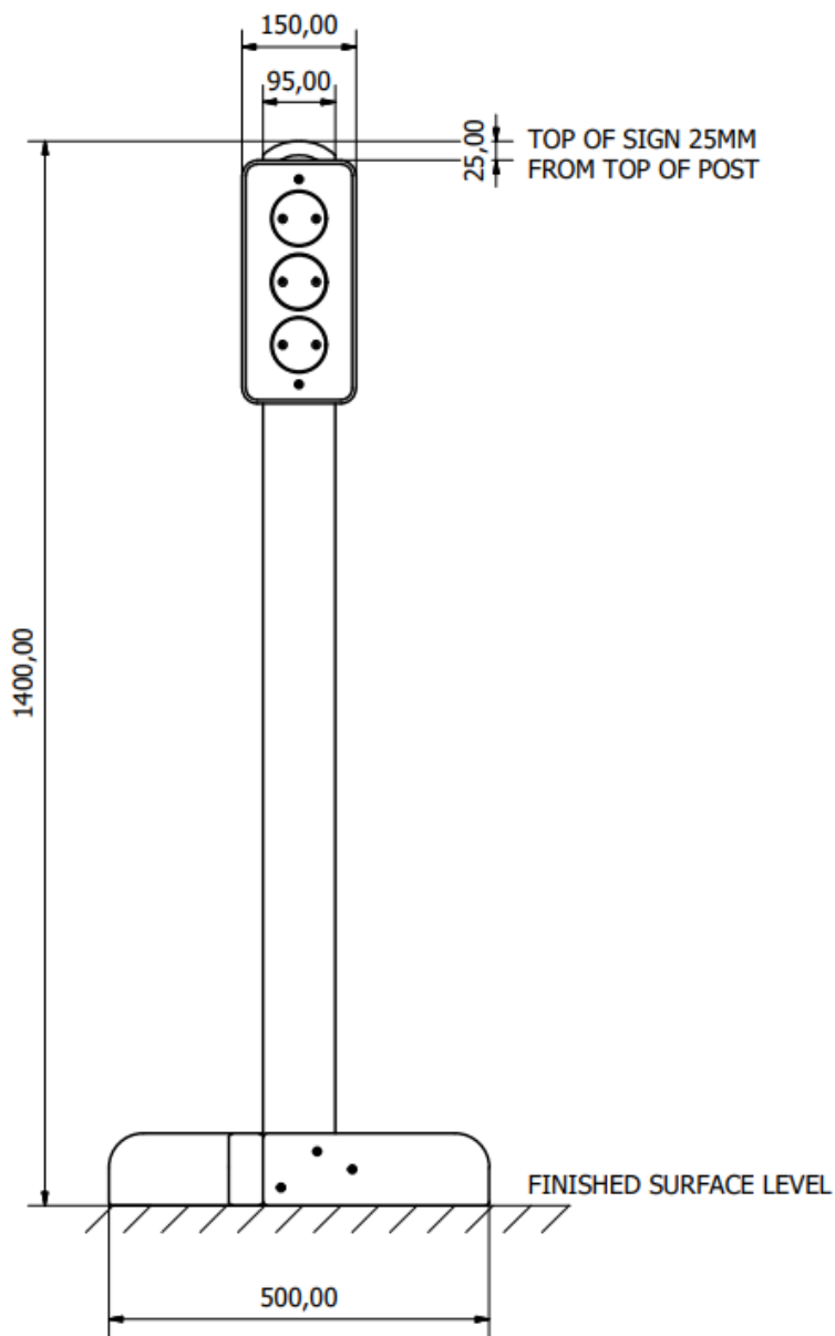
Side Elevation
